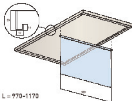
Ripiano speciale prof. 350 per cartelle sospese P 350 special shelf for suspension files with internal 330 mm hooks
