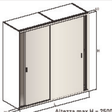
Sportelli scorrevoli Sliding doors
